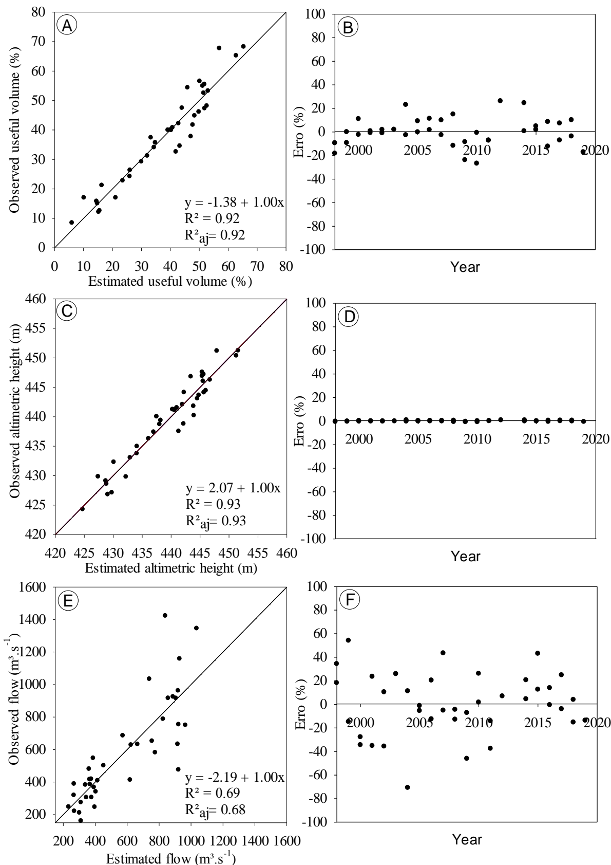
Figure 5. Relationship between observed and estimated data for variables useful volume (a) altimetric height (c) and flow (e) in wet and dry periods. Distribution of residues from the set of linear regressions for varying useful volume (b) altimetric height (d) and flow rate (F) in wet and dry periods.
