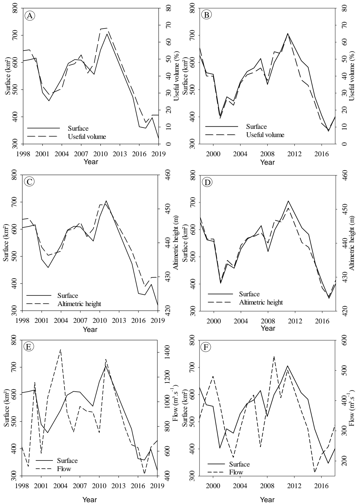
Figure 2. The relationship between the variables (A and B) useful volume (C and D), altimetric height (E and F) and flow in the wet and dry periods, respectively, for the Serra da Mesa Reservoir, GO.
