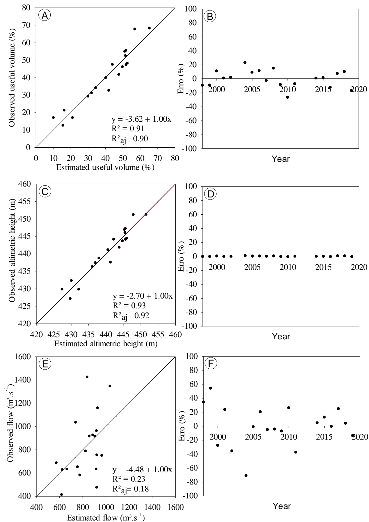
Figure 3. Relationship between observed and estimated data for the variables useful volume (A) altimetric height (C) and flow (E) in the rainy season. Distribution of residues from the set of linear regressions for variables useful volume (B) altimetric height (D) and flow rate (F) in the rainy season.
