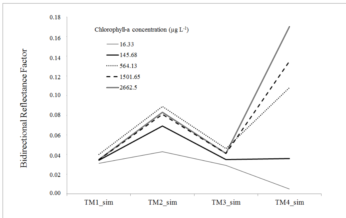
Figure 3. Bidirectional Reflectance Factor resampled to simulate Landsat/TM bands at sample stations characterized by increasing chlorophyll- \alpha concentration.
