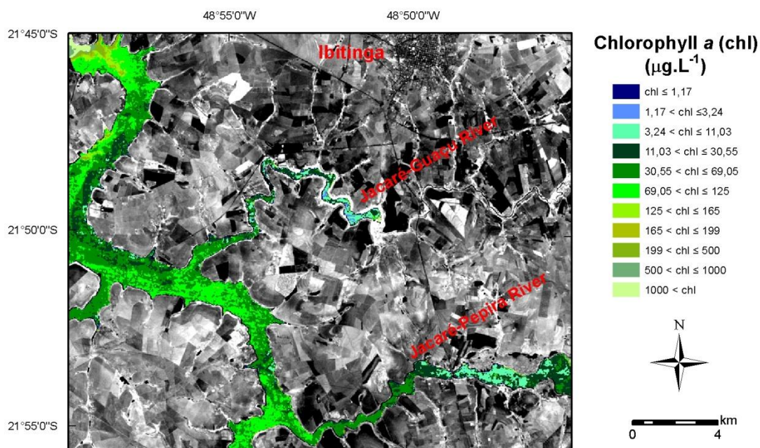
Figure 6. Reservoir inlets fed by Jacaré-Pepira River and Jacaré-Guaçu River. Chlorophyll- \alpha classification is overlying Landsat TM3 band.
